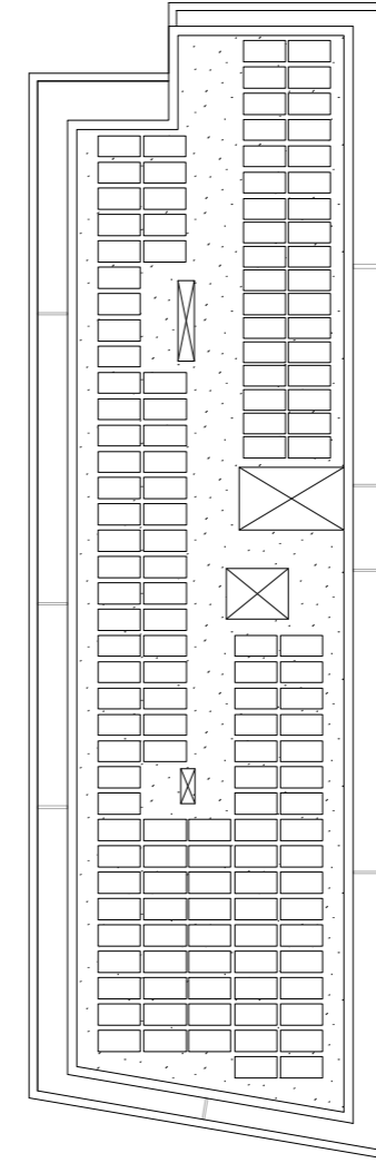
Roof plan
